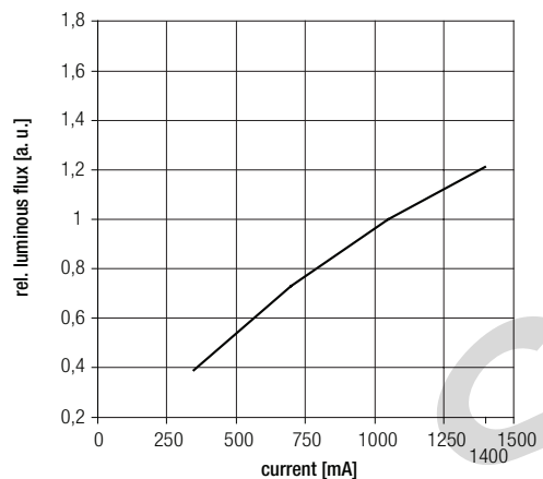
— Relative luminous flux at t_c = 65\text{ °C}
