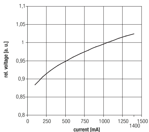
— Relative forward voltage at t_c = 65\text{ °C}
