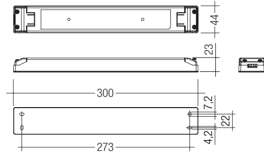
LCU 100W 12V SR top
